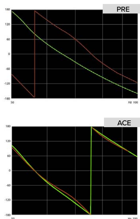
Phase Measurements of a Sub + Top Configuration taken in an Anechoic Chamber (50Hz to 100Hz window). In the 'PRE' image, no alignment was applied, while in the 'ACE' image, Top and Sub were aligned using the appropriate preset. The red curve represents the Sub phase, and the green curve the Top phase, with the Sub low-pass filter fixed at 85 Hz and the Top set to full range.
